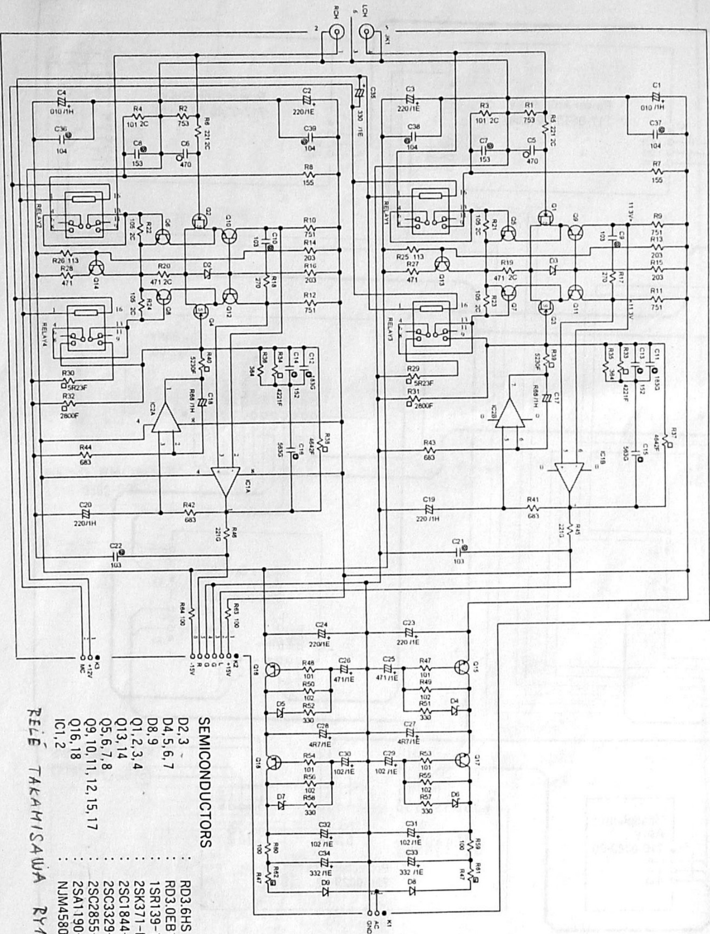
E-210 EQUALIZER ASSEMBLY (711-0034-00)
